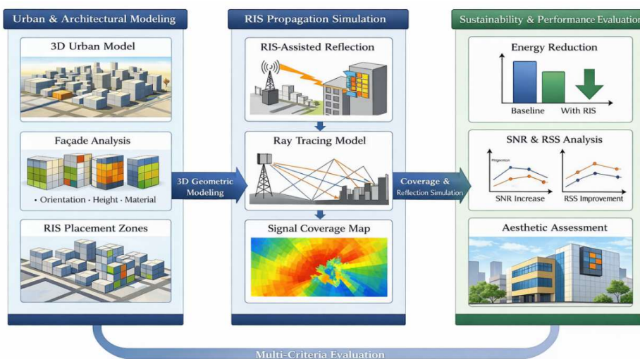
Figure 3 RIS integration in urban environments
